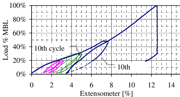
Initial to 20%, 30% & 50 % MBL & break test
